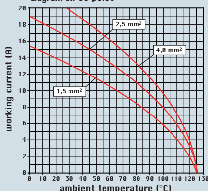
diagram CX 06 poles
