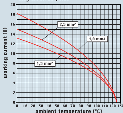
diagram CX 20 poles
