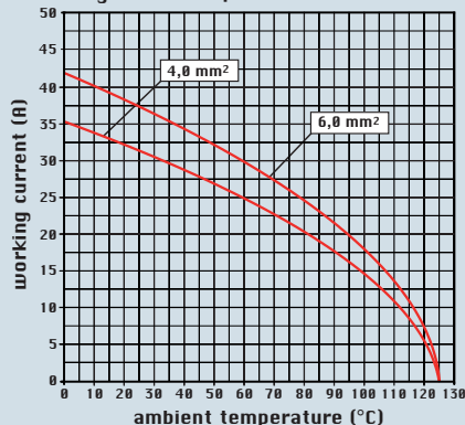
diagram CX 3/4 poles
